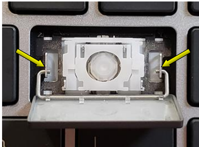
Insert stabilizer bar(s) into the appropriate brackets
